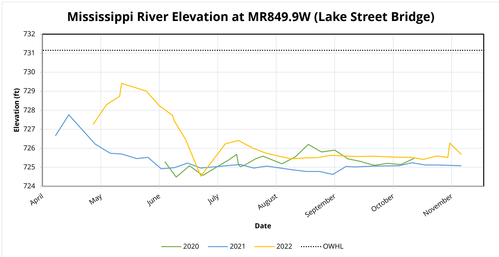
Figure 6. Mississippi River elevation values between April and November in 2020, 2021, and 2022 at river mile 849.9. Staff gage readings were collected approximately every week or when monitoring staff were on site and able to read gage. Ordinary high water level (OHWL) value included for comparison.
