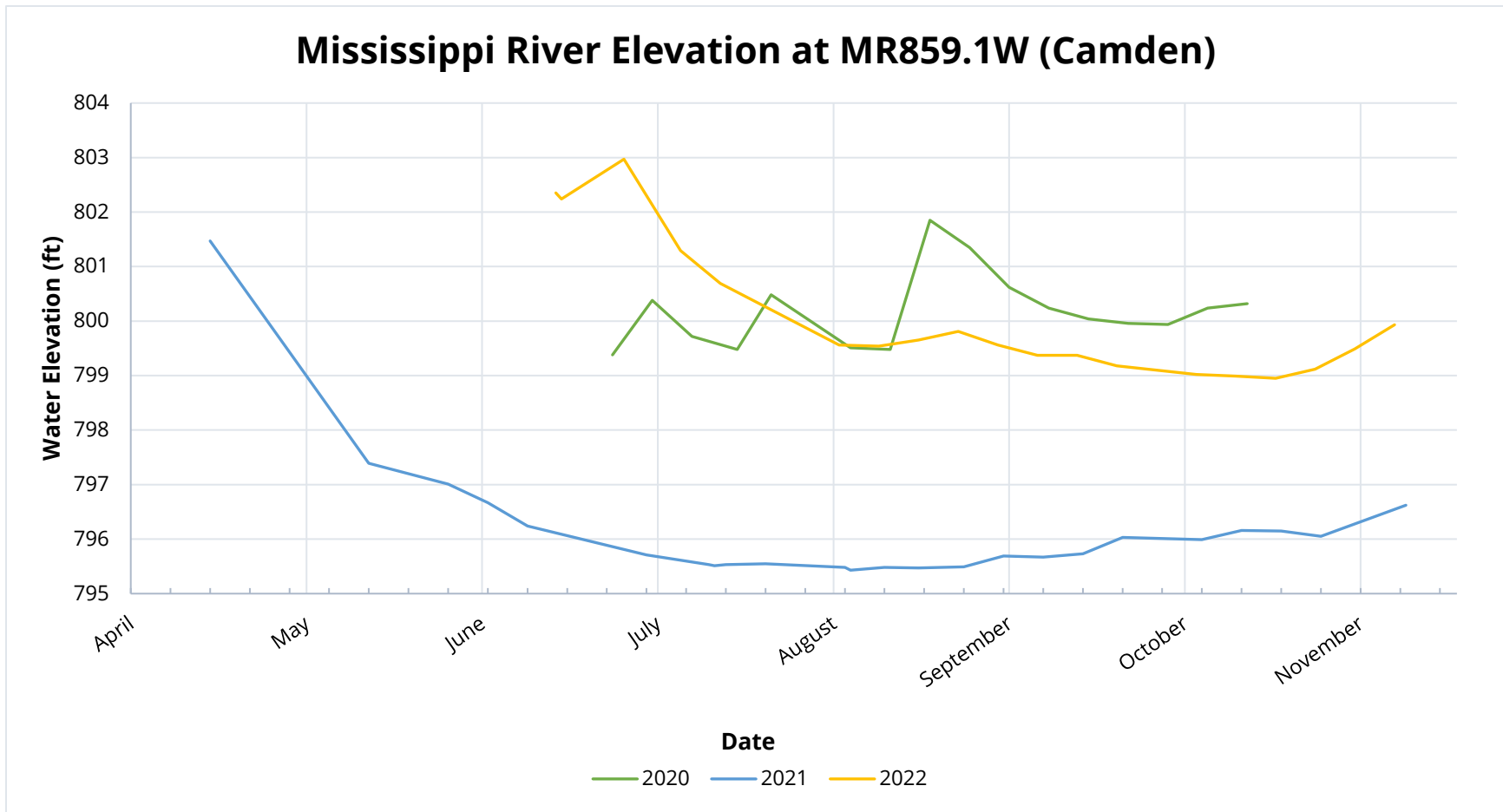
Figure 1. Mississippi River elevation values between April and November in 2020, 2021, and 2022 at river mile 859.1. Staff gage readings were collected approximately every week or when monitoring staff were on site and able to read gage.
