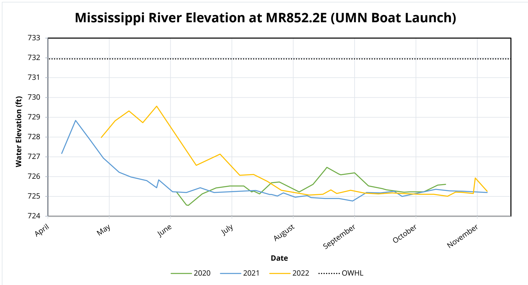
Figure 5. Mississippi River elevation values between April and November in 2020, 2021, and 2022 at river mile 852.2. Staff gage readings were collected approximately every week or when monitoring staff were on site and able to read gage. Ordinary high water level (OHWL) value included for comparison.
