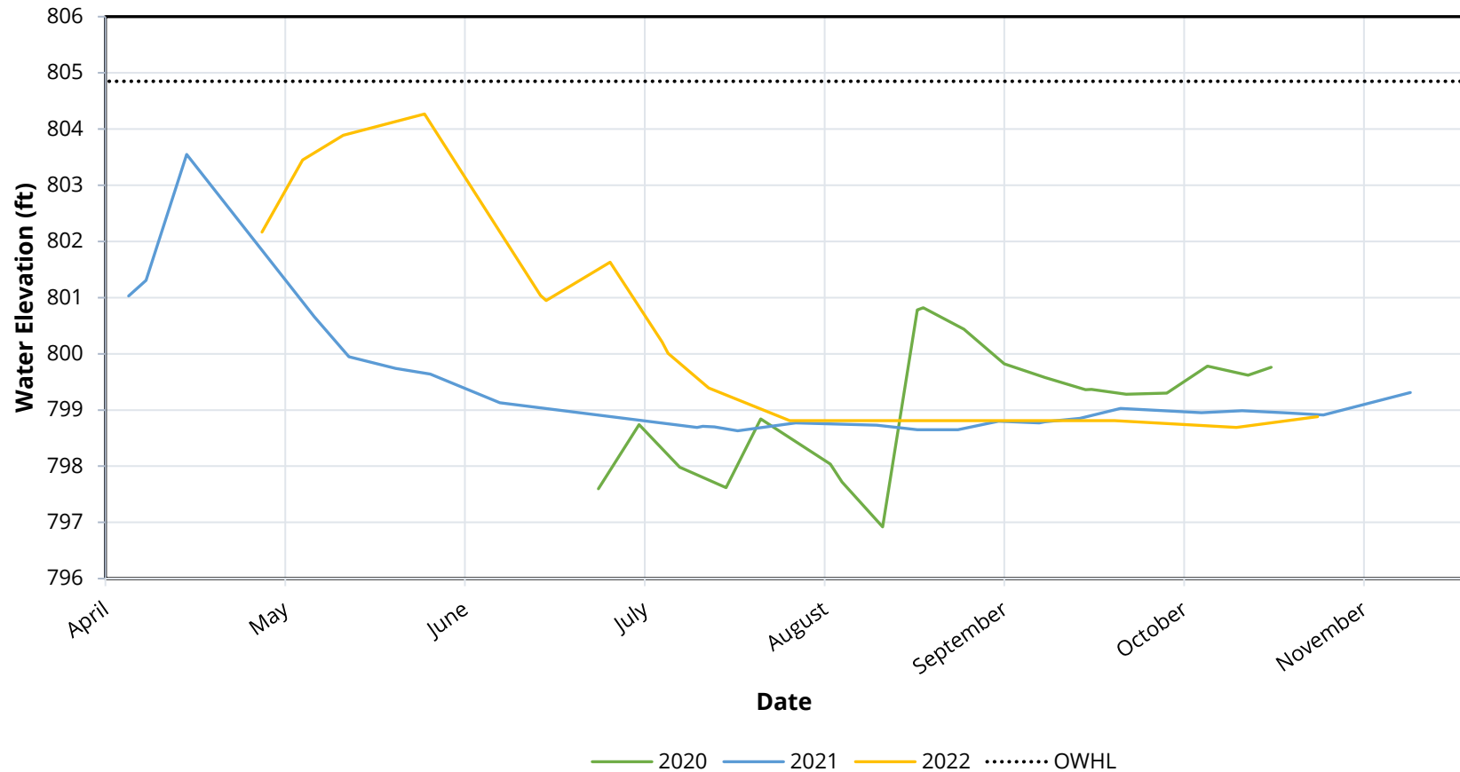
Figure 2. Mississippi River elevation values between April and November in 2020, 2021, and 2022 at river mile 857.6. Staff gage readings were collected approximately every week or when monitoring staff were on site and able to read gage.
