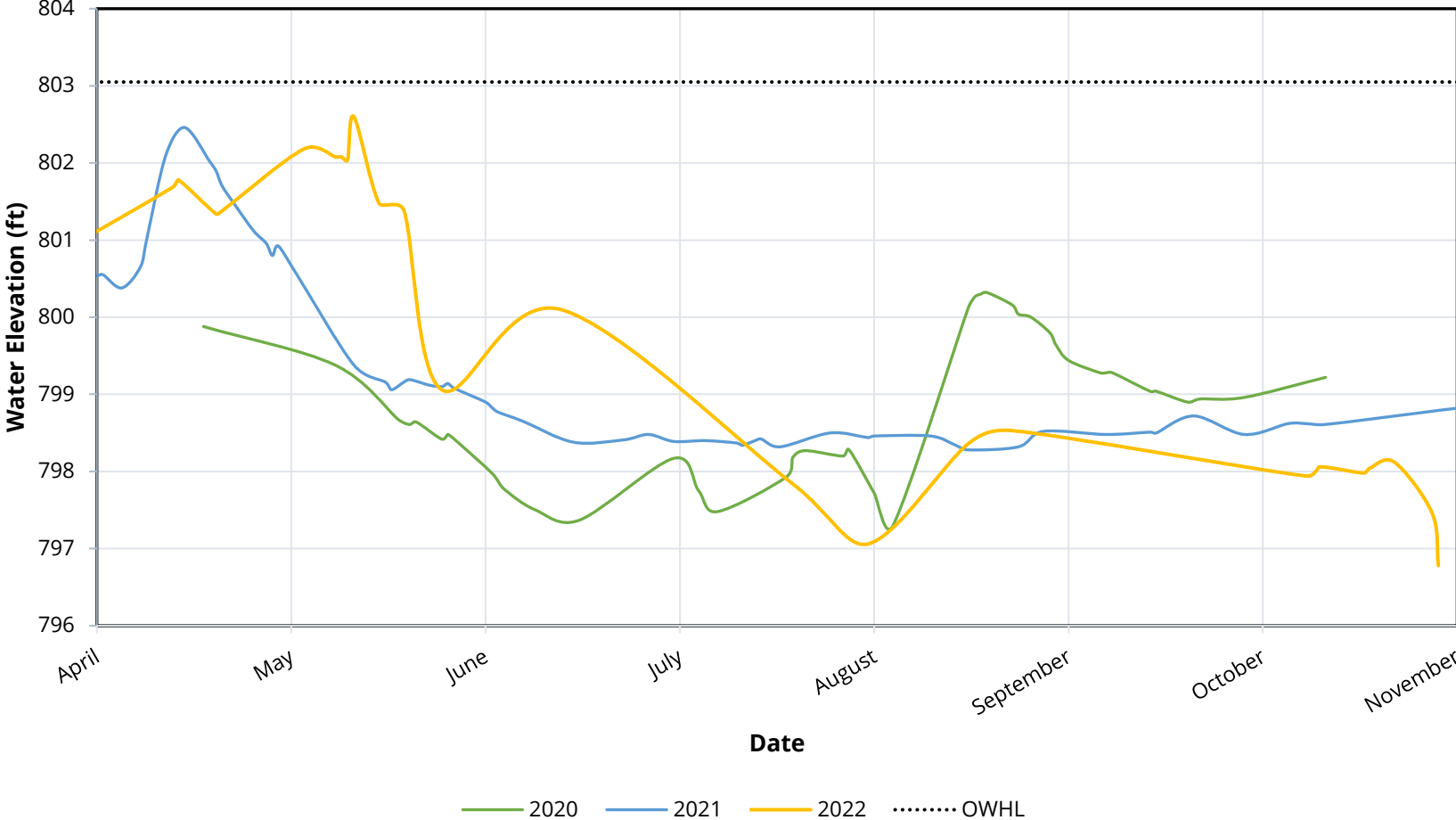
Figure 3. Mississippi River elevation values between April and November in 2020, 2021, and 2022 at river mile 856.4. Staff gage readings were collected daily Monday-Friday or when staff were available to read gage.
